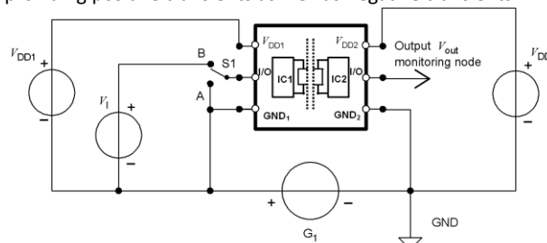
Figure 17. Common-mode transient immunity (CMTI) measurement
